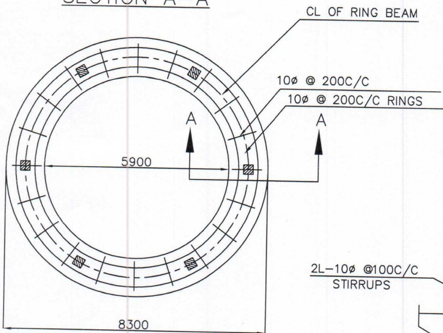
BOTTOM REINFORCEMENT OF RING FOUNDATION SBC 20t/M 2
