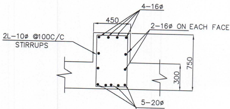
SECTION OF RAFT RING BEAM
