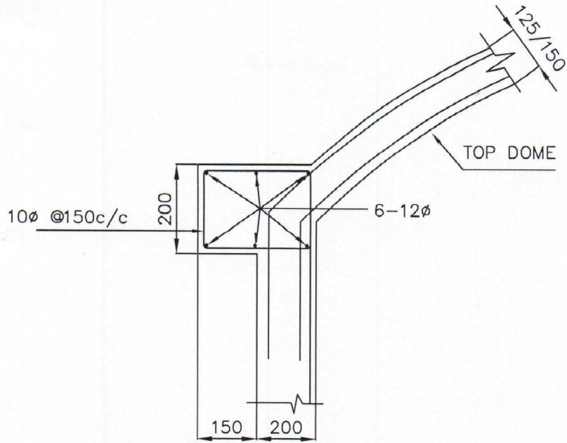
DETAILS OF TOP DOME RING BEAM
