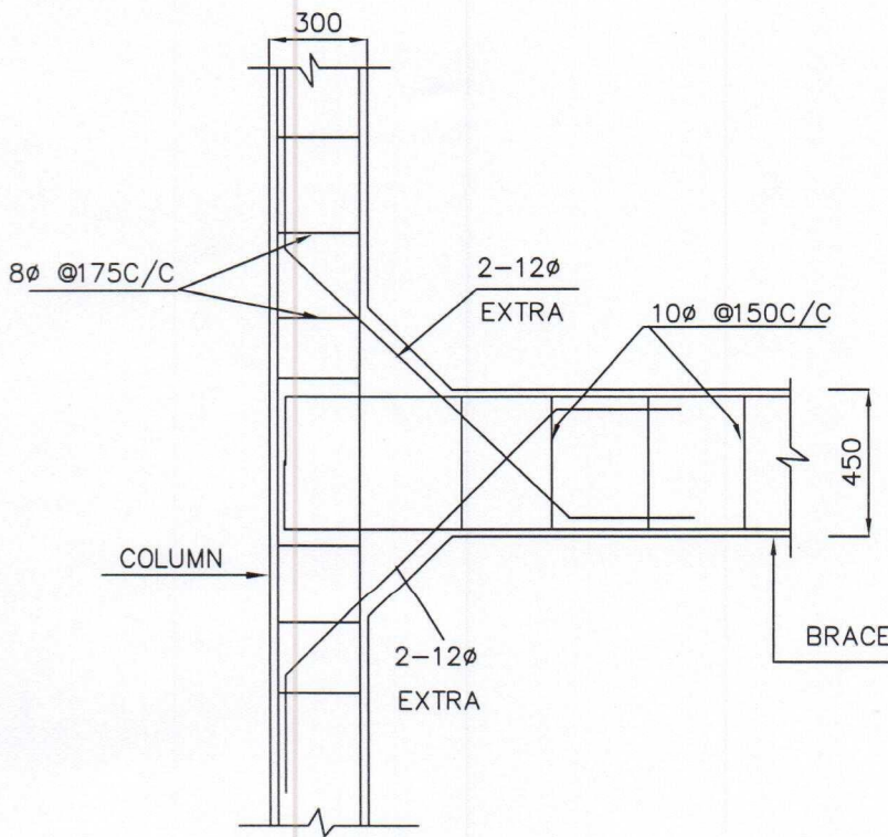
COLUMN BRACE JUNCTION
