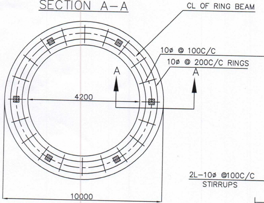
BOTTOM REINFORCEMENT OF RING FOUNDATION SBC 7.5t/M 2
